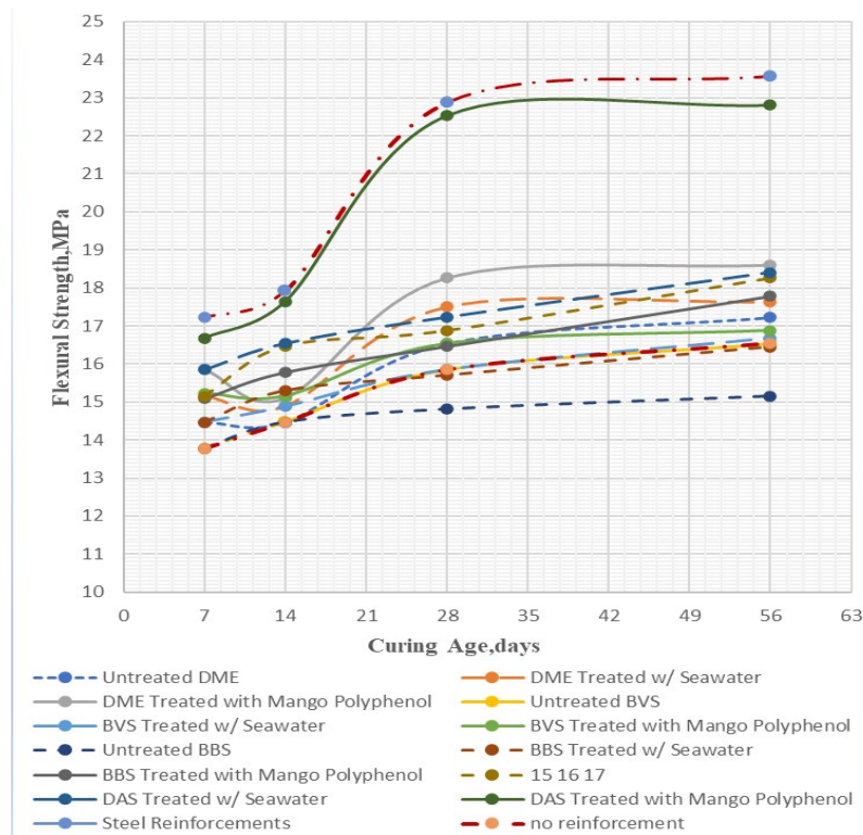
Fig. 3. Flexural Strength of Concrete beam reinforced with bamboo sticks as a replacement for Steel bars.
