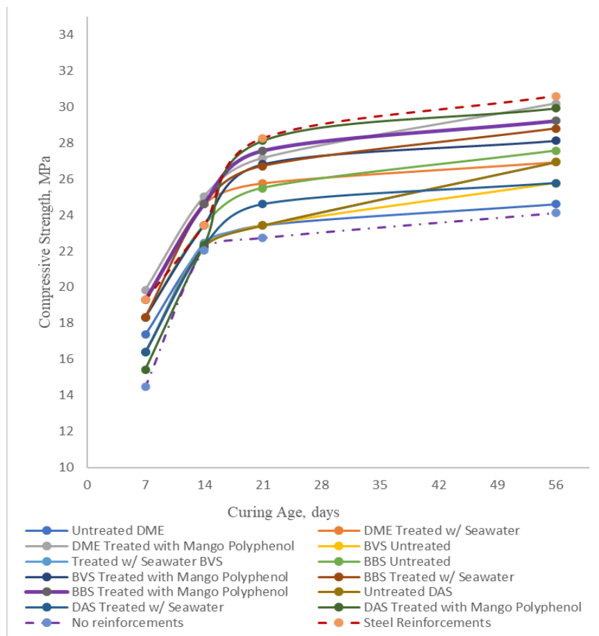
Fig. 2. Compressive Strength of Concrete Reinforced with bamboo sticks as a replacement for Steel bars.
