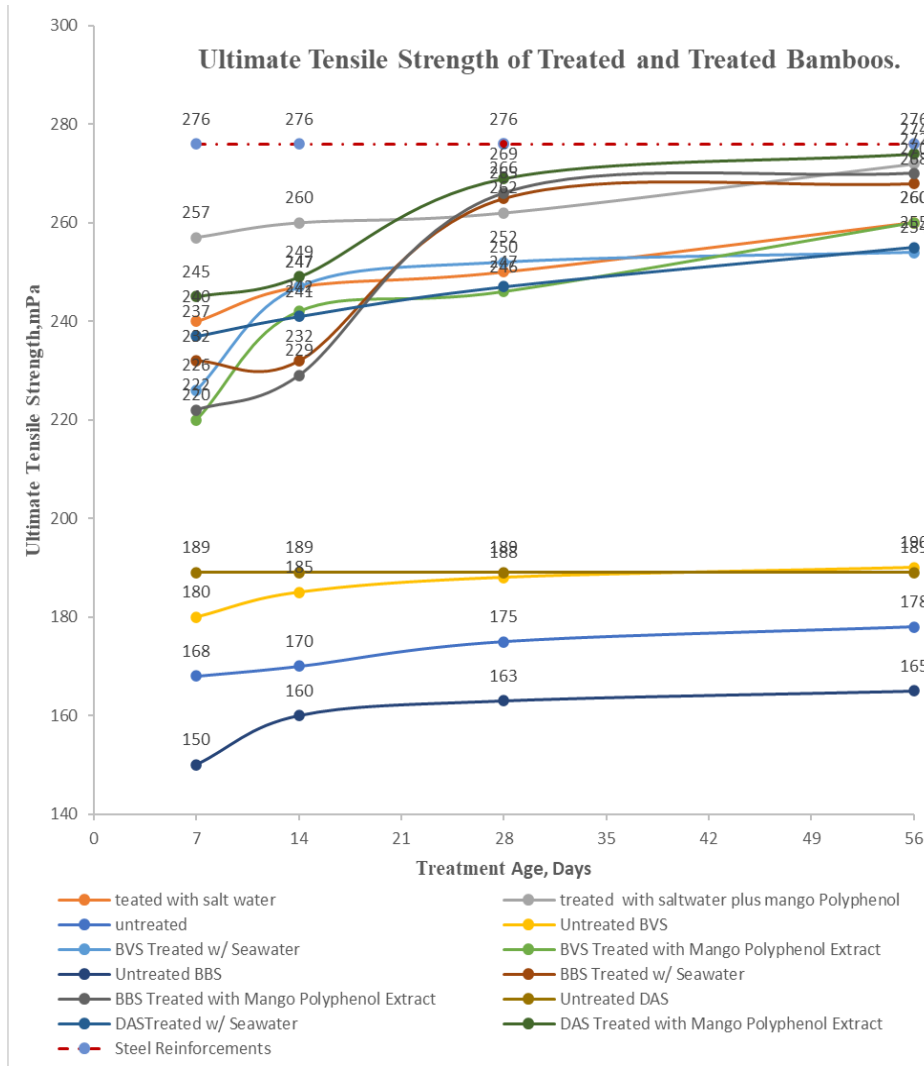
Fig.1. Ultimate Tensile Strength of Bamboo Specimen Sticks
